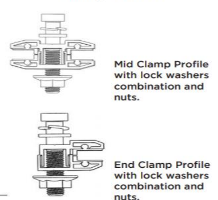
Clamp Profiles
