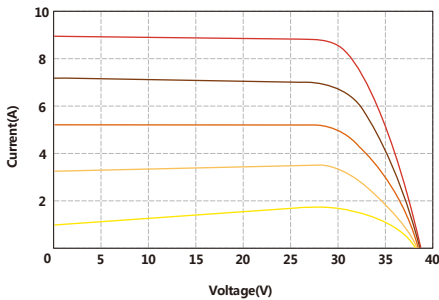
Current-Voltage & Power- Voltage Curve (AD270M4-Ab)
