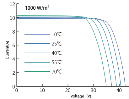
Current-Voltage Curve under different working temperatures
