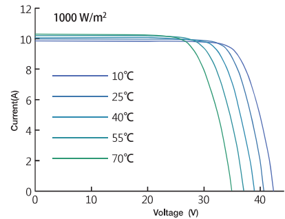
Current-Voltage Curve under different working temperatures
