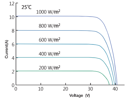
Current-Voltage Curve under different irradiance
