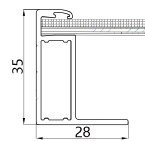
Section A-A Dimension (unit: mm)
