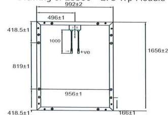
Drawing of 25560 - 275 Wp Module
