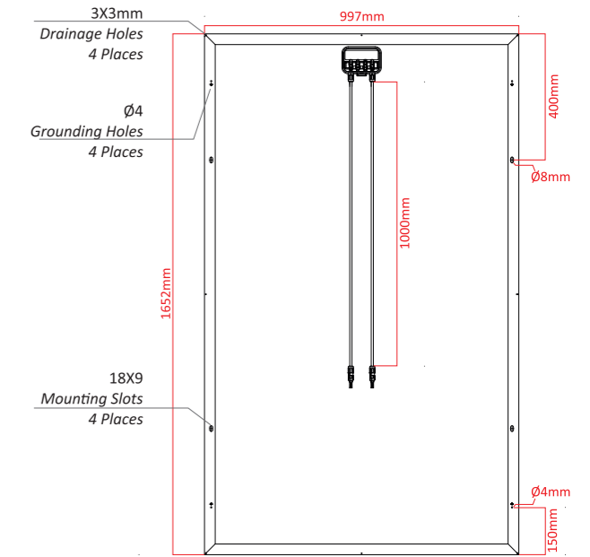
FRAME CAN BE MANUFACTURED WITH TWO DIFFERENT MEASUREMENT OPTIONS.
