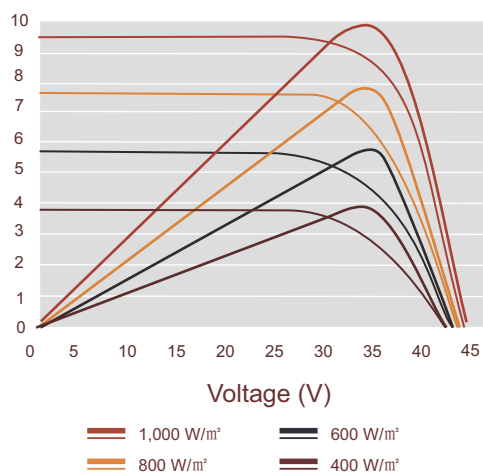
I-V Curves at Different Irradiances (330W) Test Temperature: 25°C
