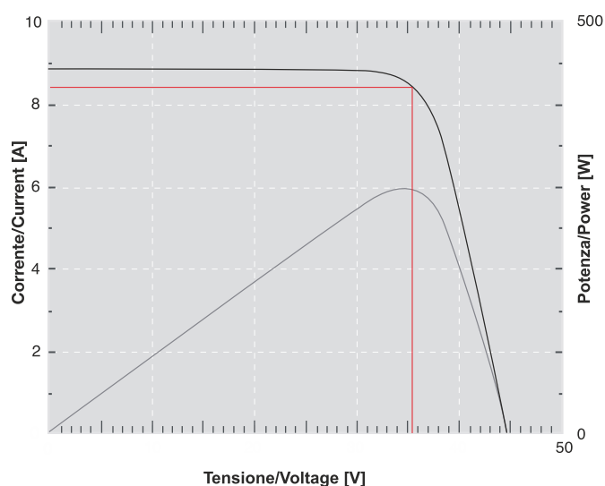
Curve Corrente/Tensione e Potenza/Tensione (modulo Micron 72M da 300 Wp) Current/Voltage and Power/Voltage Curves (300 Wp Micron 72M module)
