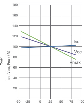
Temperature coefficient
