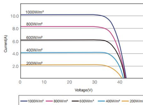
I-V CURVES OF PV MODULE(315W)
