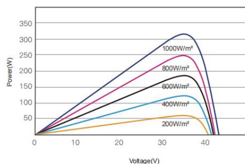
P-V CURVES OF PV MODULE(315W)
