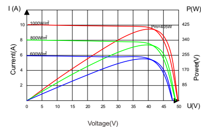
Current-Voltage&Power-Voltage Curve(405W)
