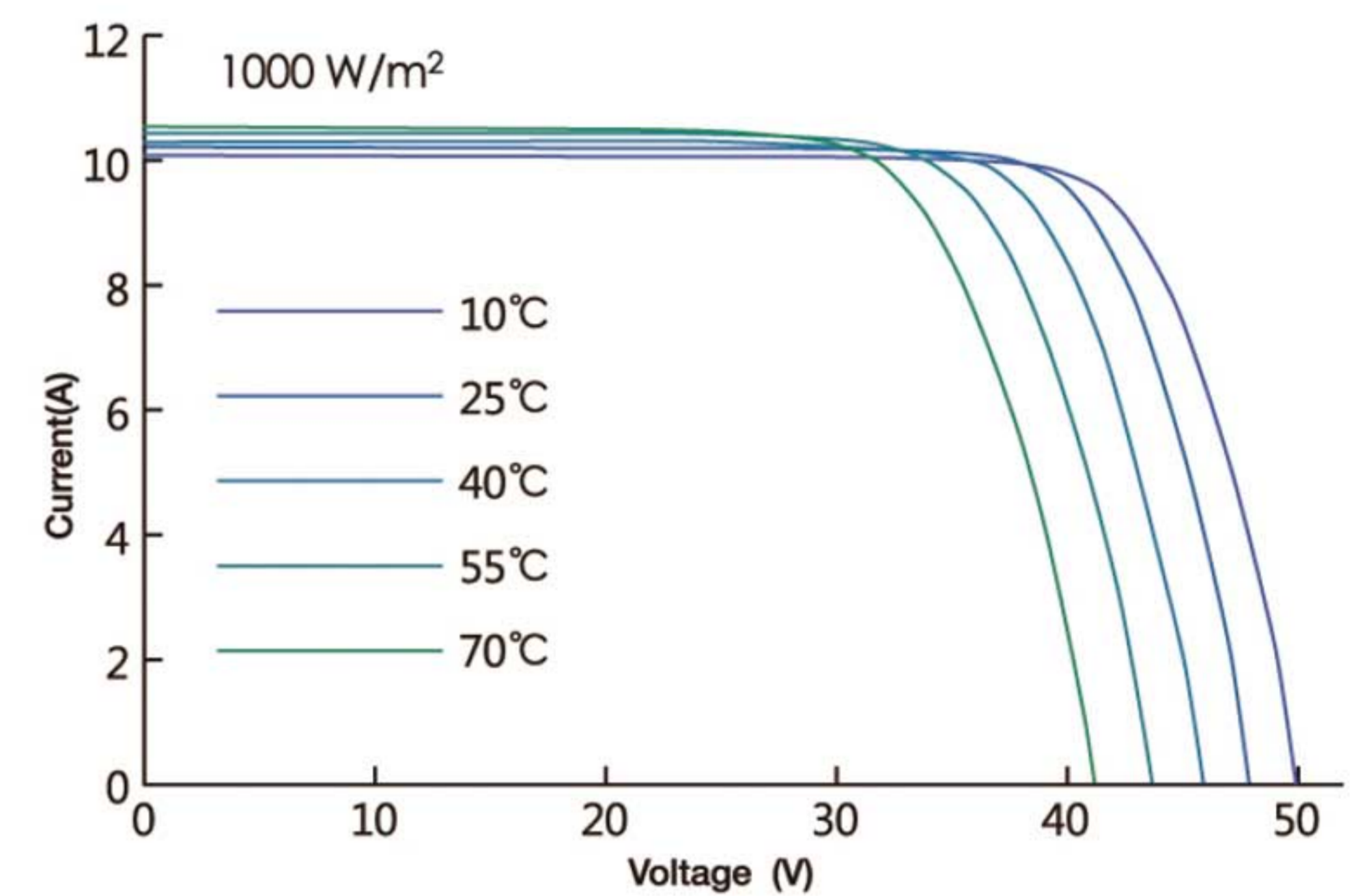
Current-Voltage Curve under different working temperatures
