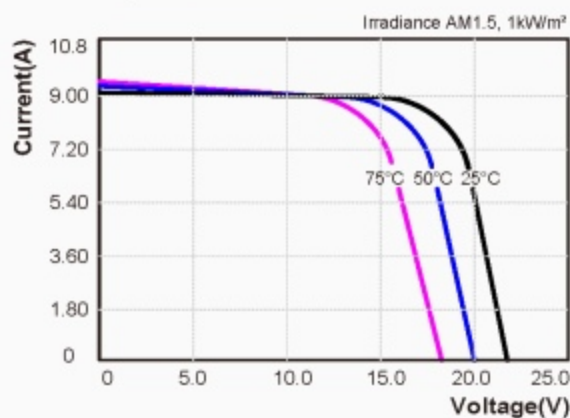
I-V Curves of PV module ESF150PA at various cell temperatures
