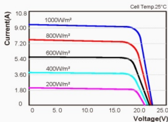
I-V Curves of PV module ESF150PA
