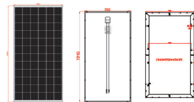
Engineering Drawing
