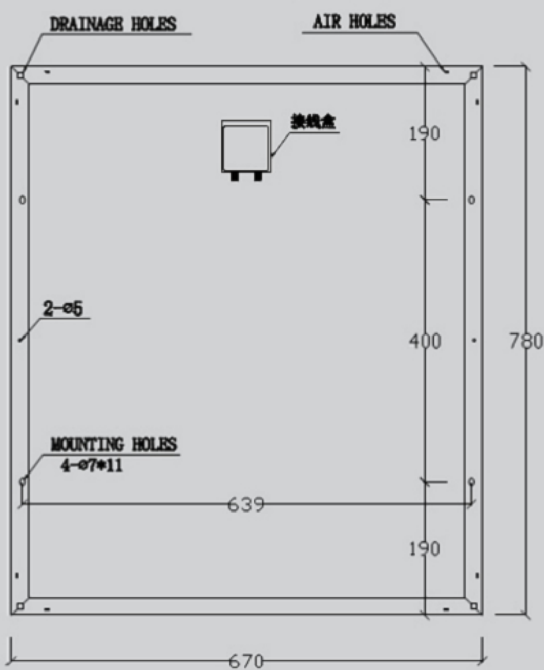
Engineering Drawings (Back Side)
