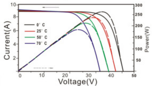
Irradiance:AM1.5,1000W/m 2
