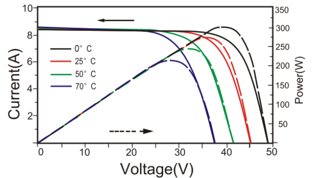
Irradiance:AM1.5,1000W/m²
