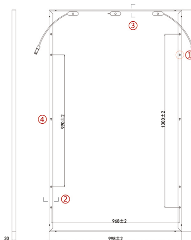
ENGINEERING DRAWING ( unit : mm )
