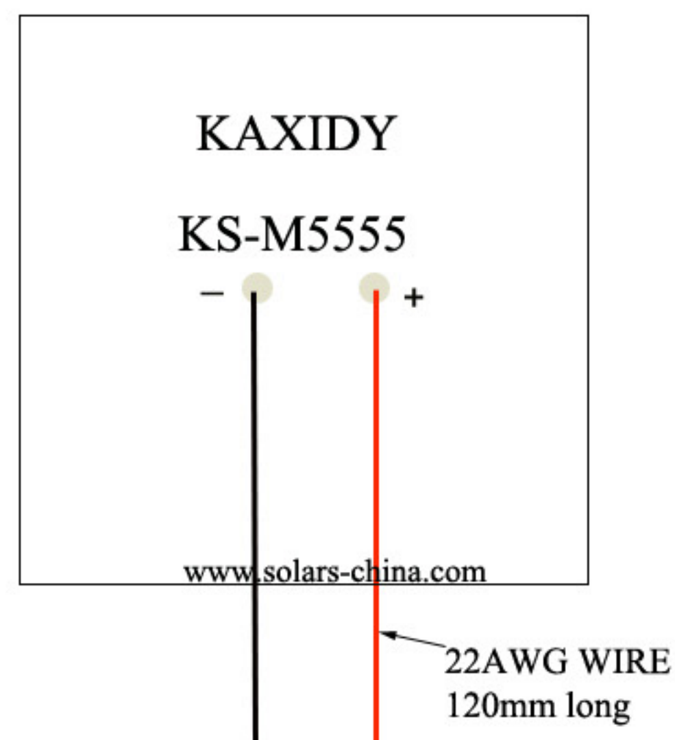
BACK VIEW
