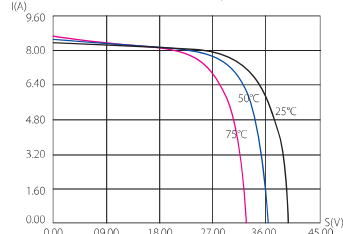
I-V curve under different temperature
