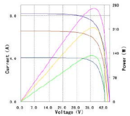
Current, power VS voltage characteristics (solar irradiant 100%, 80%, 50%)
