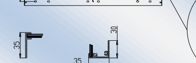
A-A' section B-B' section
