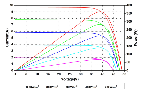
Current-Voltage & Power-Voltage Curves At Different Irradiances
