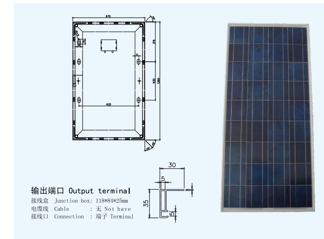
YHM120-18P
